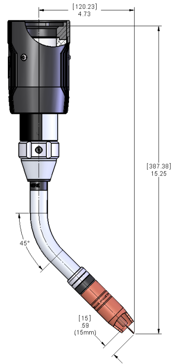
45° Gooseneck, Part # 59G45L – 0.59" (15 mm) CTWD
